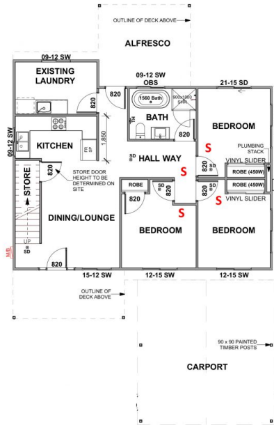
GROUND FLOOR PLAN 1:100
