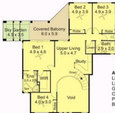
Upper Level
