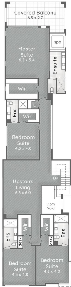
:: FLOOR PLAN First Floor - 3.0m Ceiling
