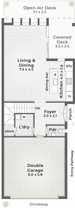
:: GROUND FLOOR 2.5m Ceiling
